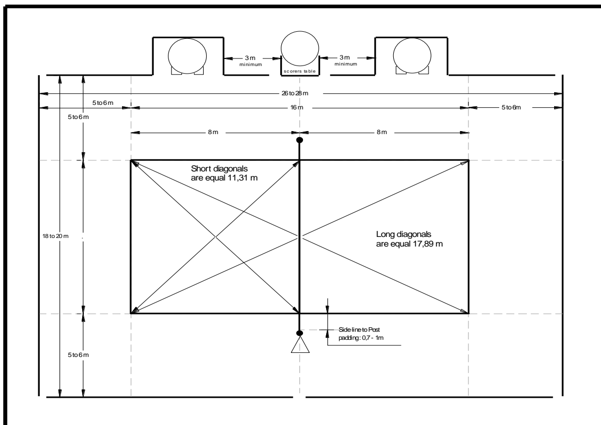
Court Layout - Fig. 1
